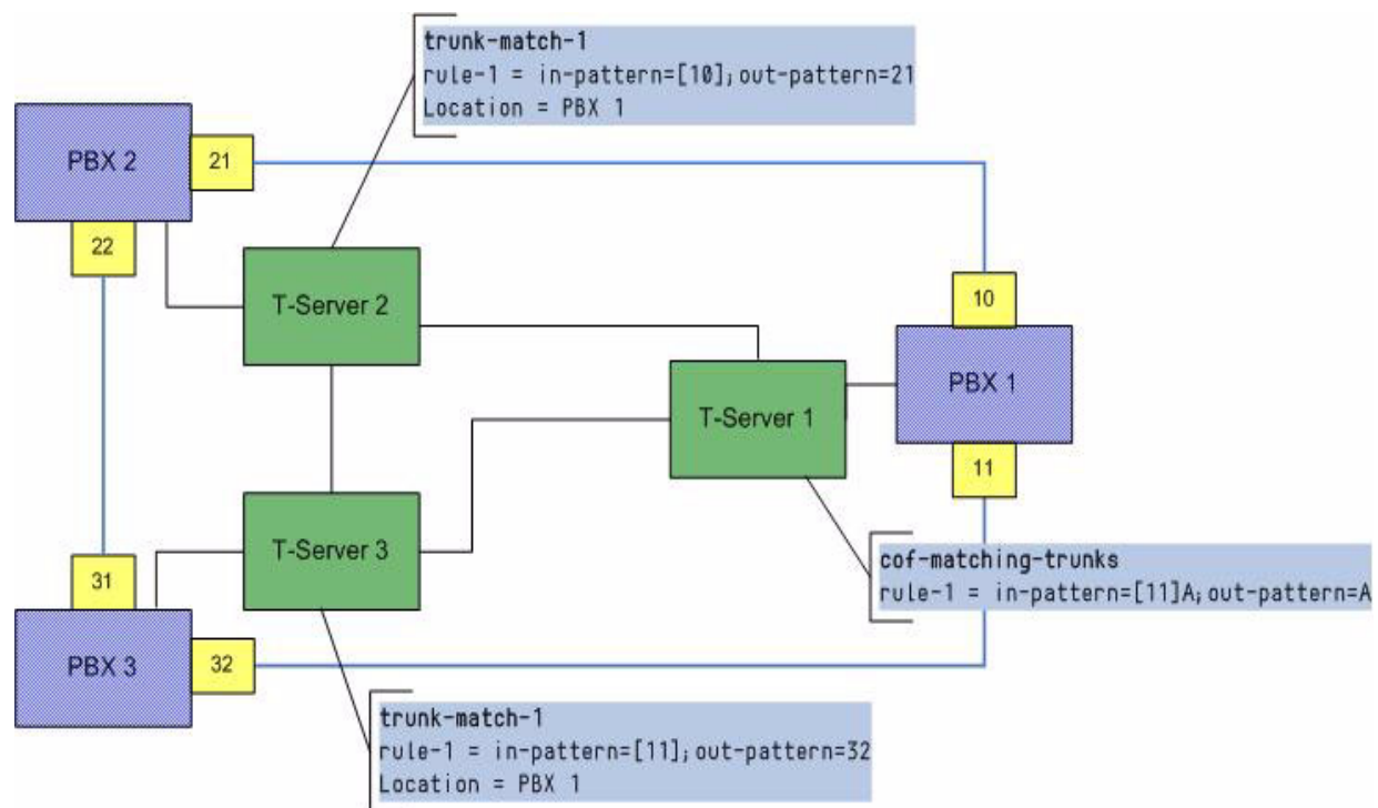
Figure 14: Flexible Trunk Matching—T-Server Configuration Schematic
