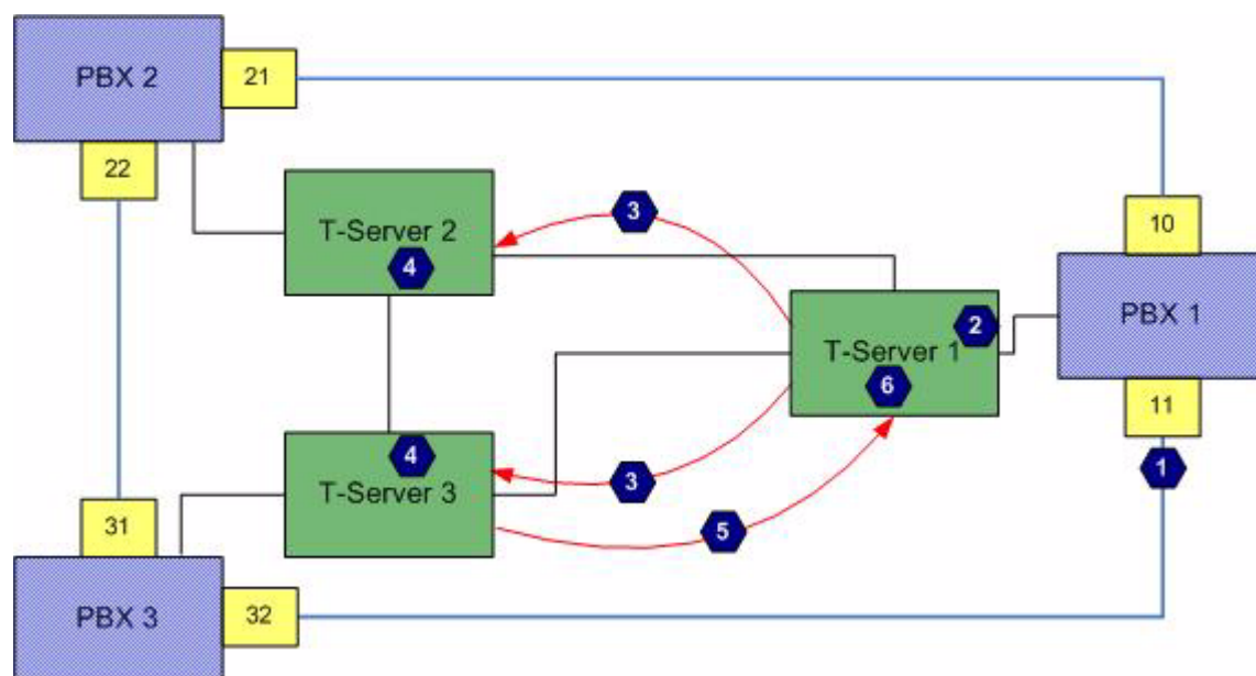
Figure 13: Flexible Trunk Matching—Process Flow
