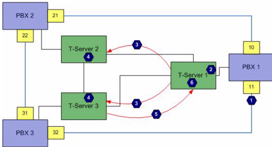
Figure 12: Flexible Trunk Matching—Process Flow
