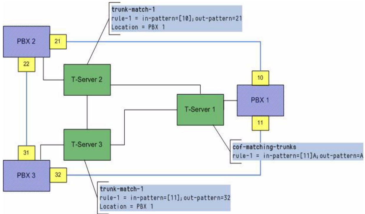
Figure 13: Flexible Trunk Matching—T-Server Configuration Schematic
