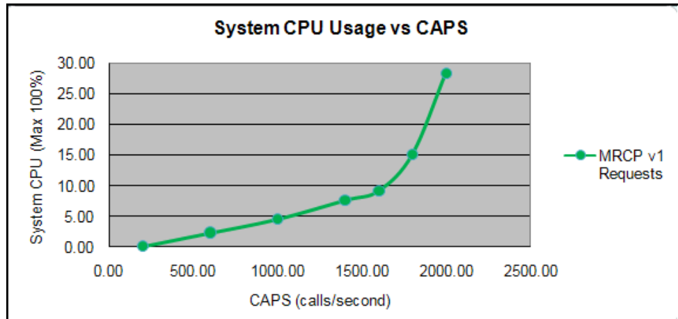
Figure 127: System CPU Usage Versus CAPS—MRCPv1 (MRCP Proxy)
