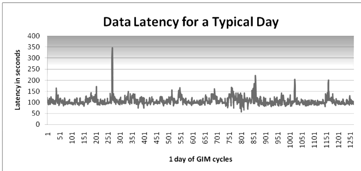
Figure 34: Data Latency—Endurance Test
