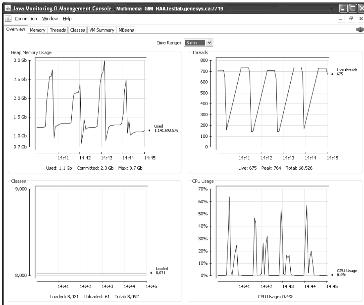
Figure 40: JVM Activity
