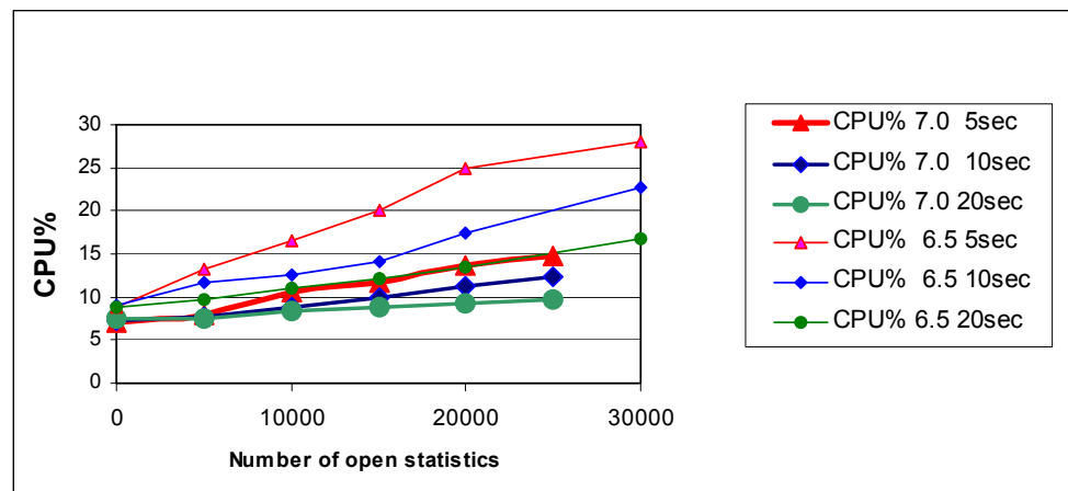
Figure 171: Stat Server Performance Improvements 7.0 vs. 6.5
