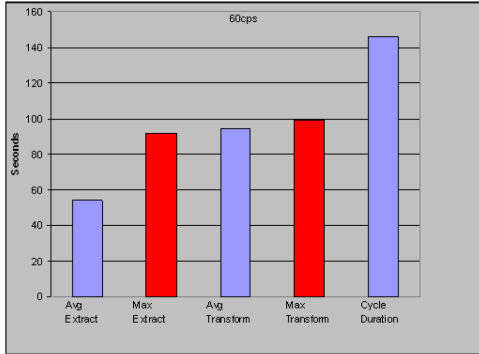
Figure 71: Extraction and Transformation Times—60 cps
