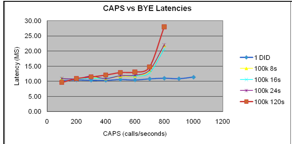
Figure 122: CAPS Versus SIP BYE Latencies (Resource Manager)
