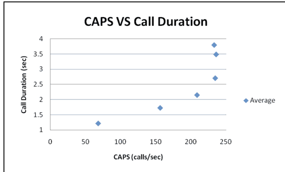
Figure 92: CAPS Versus CD (Average)
