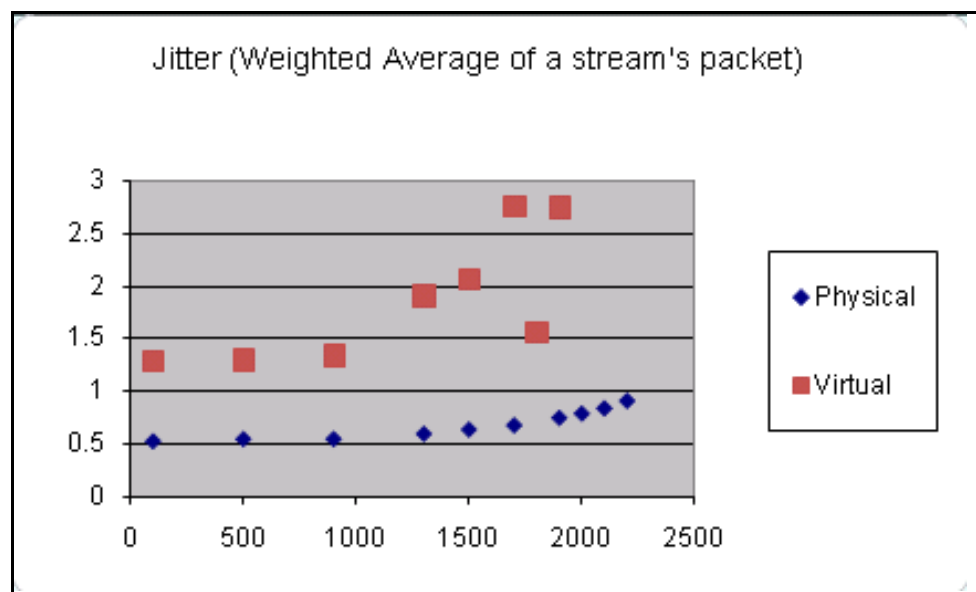
Figure 147: Jitter (Weighted Average)
