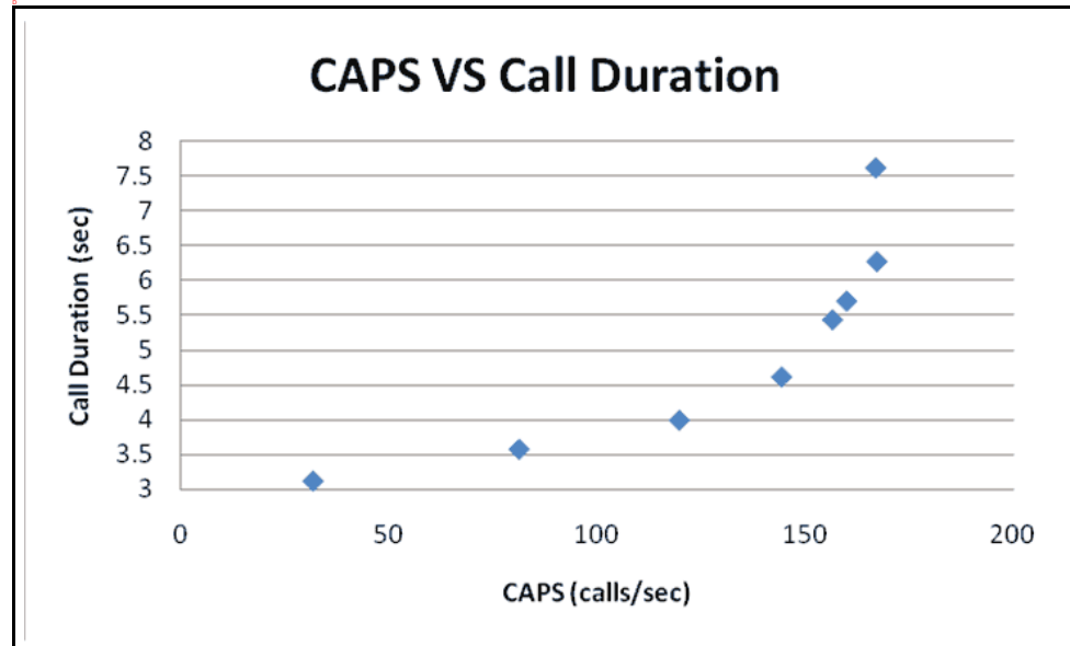
Figure 90: CAPS Versus CD (Announcement)
