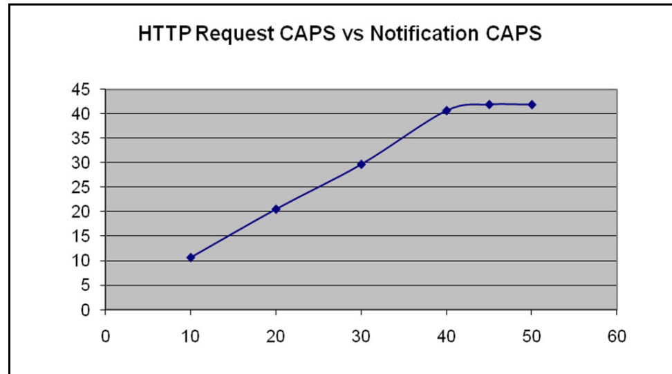
Figure 132: HTTP Request CAPS Versus Notification CAPS
