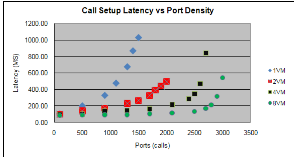
Figure 137: Call Setup Latency Versus Port Density (Virtual Machines)
