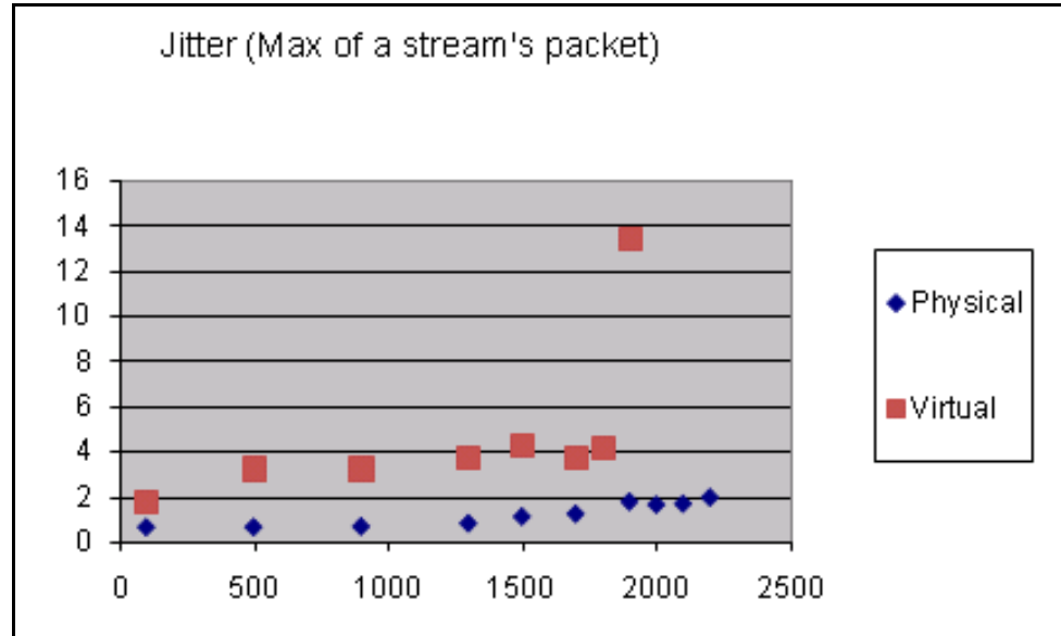
Figure 148: Jitter (Maximum of Streamed Packets)
