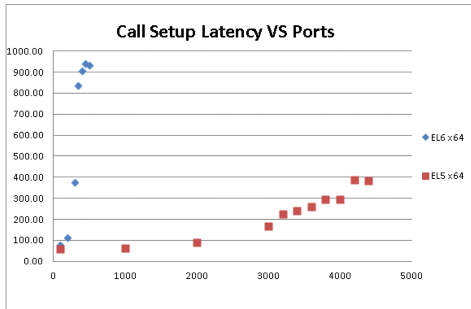
Figure 116: Call Setup Latency vs. Ports
