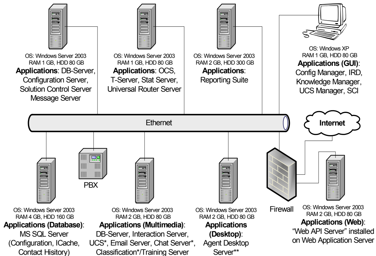
Figure 1: Sample eServices (Multimedia) Architecture
