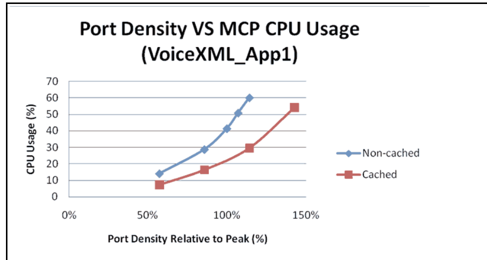
Figure 88: PD Versus CPU (VoiceXML_App1)
