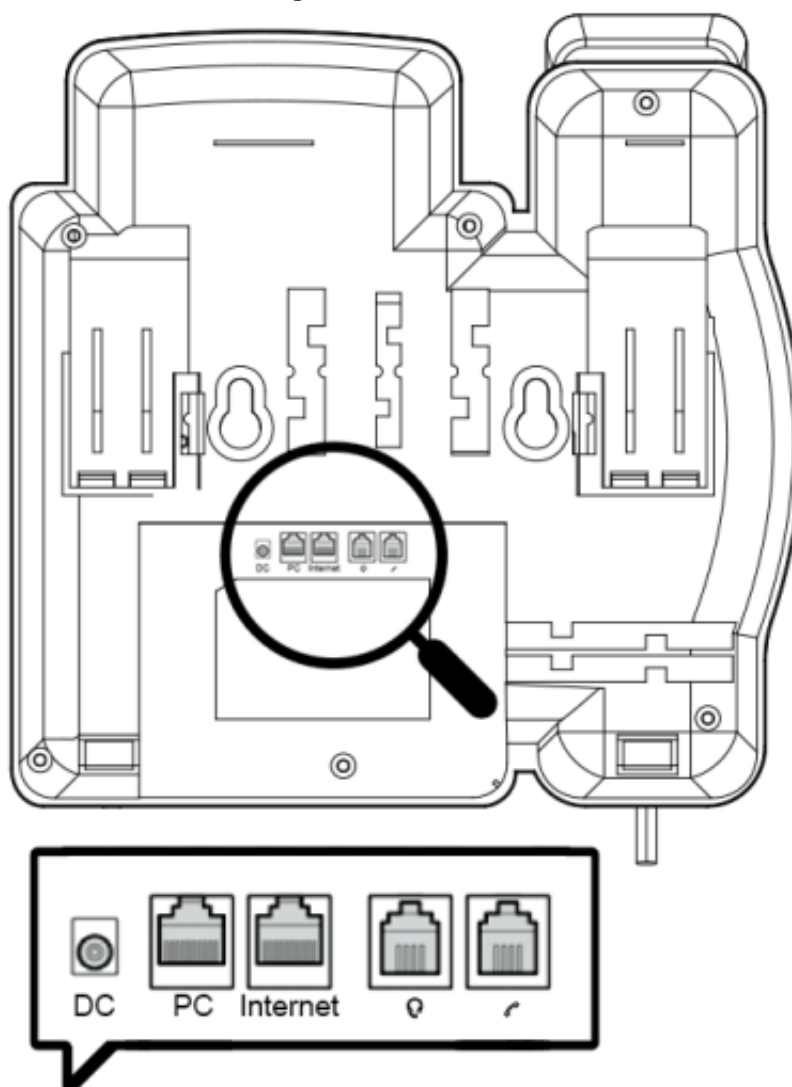
Figure 2-2: Rear View
